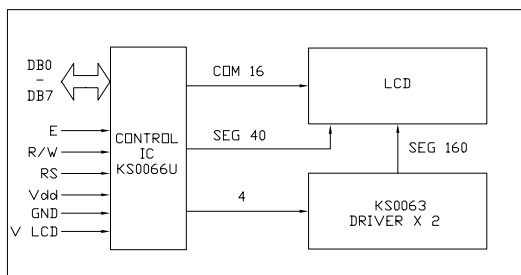
STANDARD CONFIGURATION
