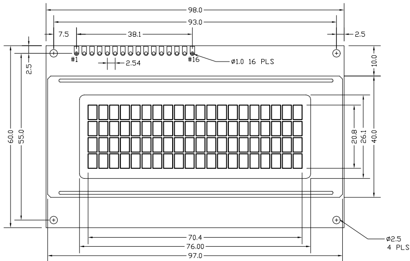
STANDARD CONFIGURATION
